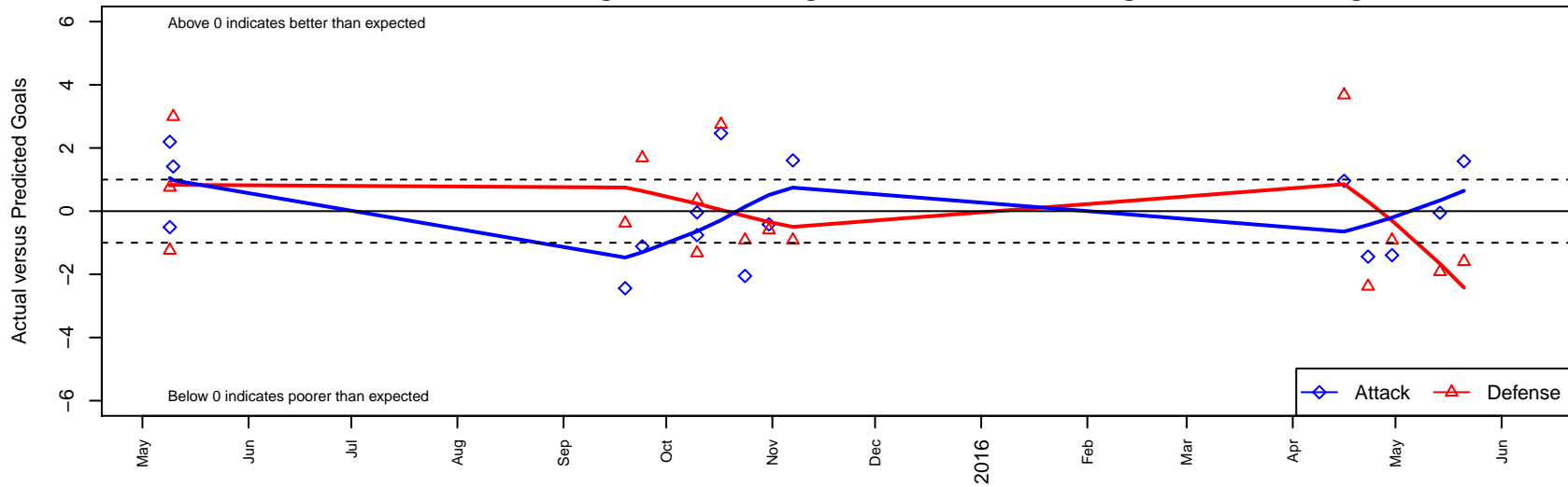
Moscow United B03 Dots are actual minus expected GF (blue circles) and GA (red triangles). Blue line is smoothed change in attack strength. Red is smoothed change in defense strength.
